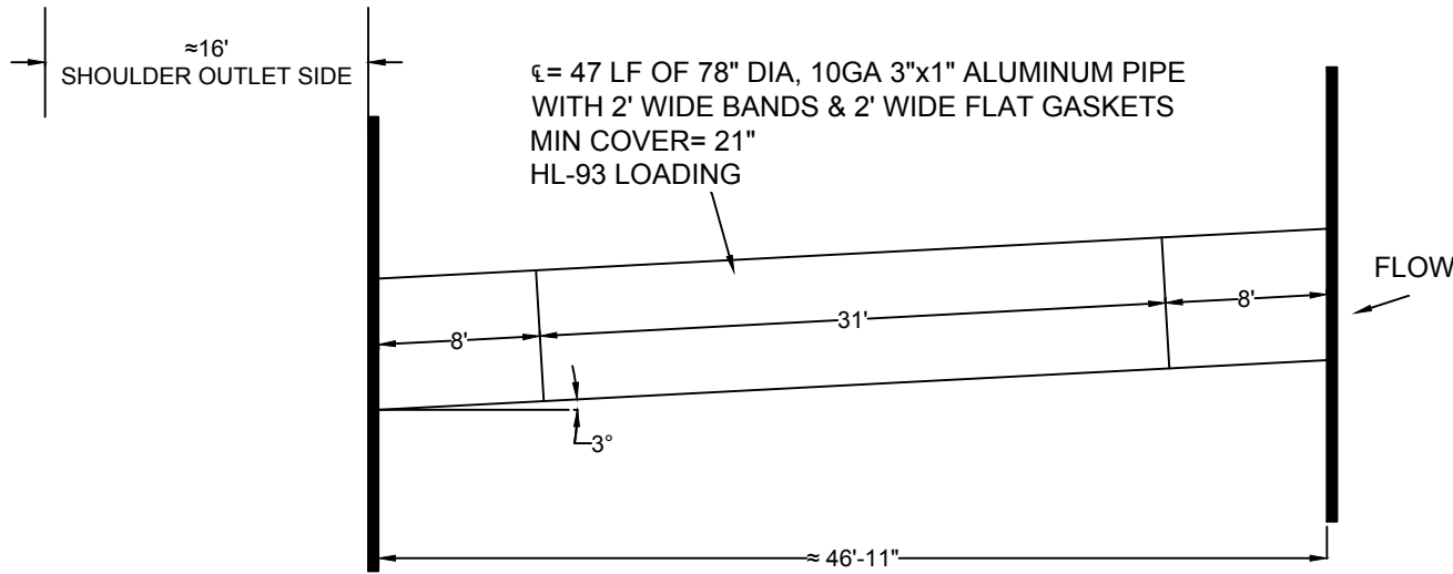
PLAN VIEW
