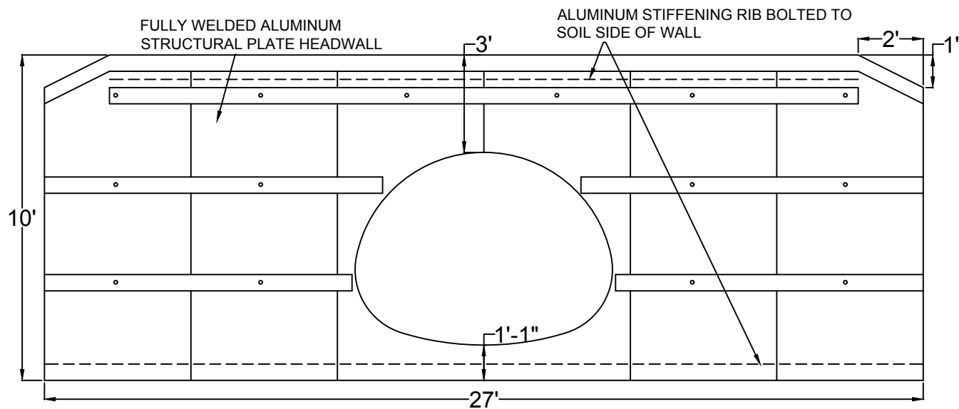
END VIEW- INLET HEADWALL
