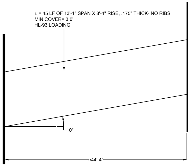
PLAN VIEW
