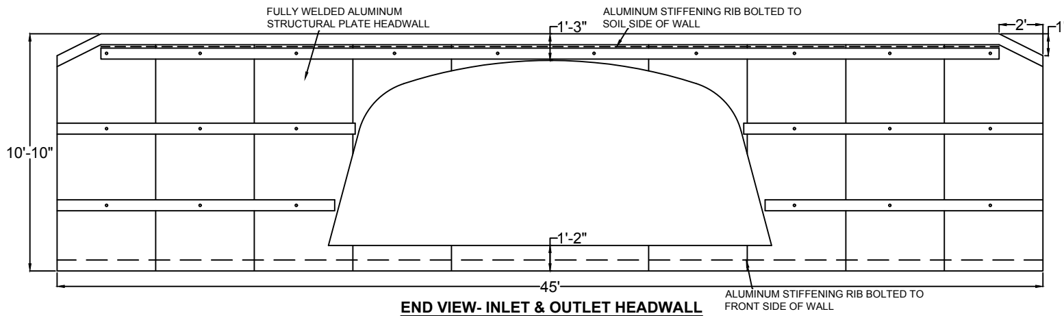
END VIEW- INLET & OUTLET HEADWALL
