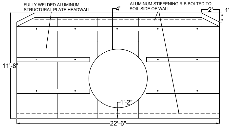
END VIEW- OUTLET HEADWALL
