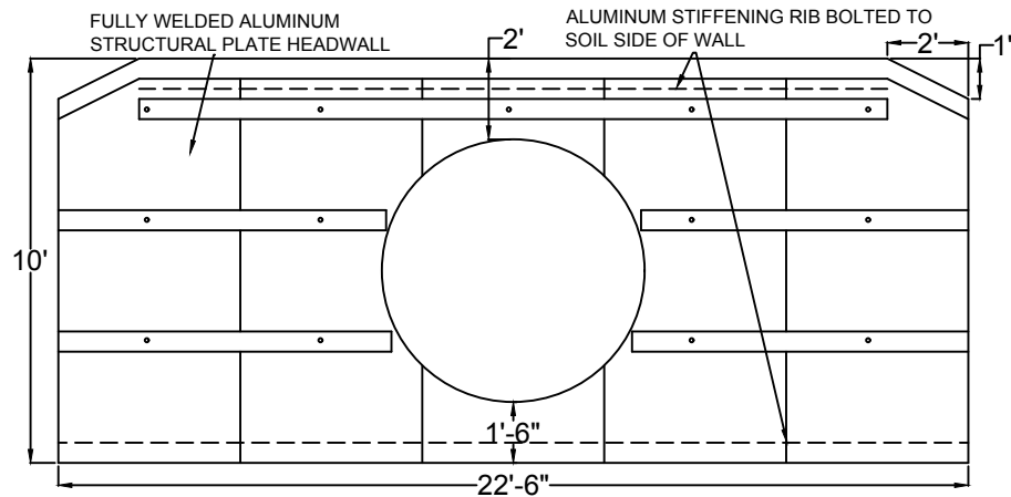
END VIEW- INLET HEADWALL
